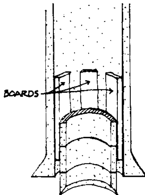
FIG. 9-6. BOARDS USED TO GUIDE SINKING RINGS
