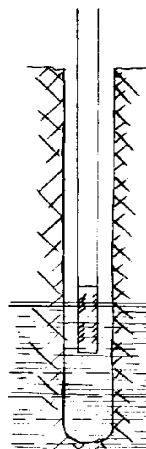
FIG. 15-8. SCREEN AND CASING BAILED DOWN
