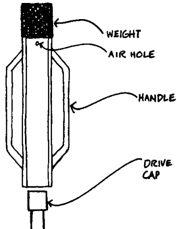
FIG. 14-7. STEEL DRIVING BAR ARRANGEMENT
