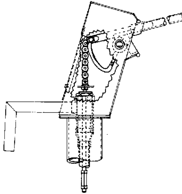
FIG. VII-8. LOCALLY MADE VARIATION OF JALNA PUMP
