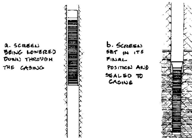
FIG. 15-6. TELESOPING SCREEN
